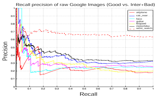
Figure 5: Recall precision curves of the raw output of Google’s image search for the 7 keywords. Good labels count as positive examples while Intermediate and Junk labels are negative examples. Note the precision drops rapidly as the recall increases, leveling out at 20–30% for most categories.
