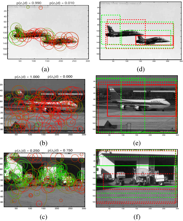
Figure 4: (a)-(c) Two airplane and one background image, with regions superimposed, coloured according to topic of a learnt pLSA model. Only a subset of regions are shown for clarity. (d)-(f) The same images as in (a)-(c) but showing the bounding boxes proposed by the pLSA model with dashed lines. The solid rectangle shows the centroid with highest likelihood under a TSI-pLSA model, with the colour indicating topic (the red topic appears to select airplanes). (d) shows multiple instances being handled correctly. (e) shows the object being localized correctly in the presence of background clutter.
